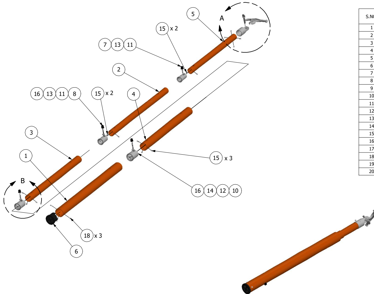
ISOMETRIC VIEW
