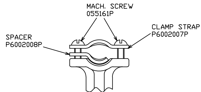
VIEW "A-A"
